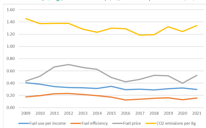
Figure 32 Evolution of Fuel intensity (l/kg), Fuel efficiency (%), Fuel use per income (l/€) and Fuel price for 2009–21
