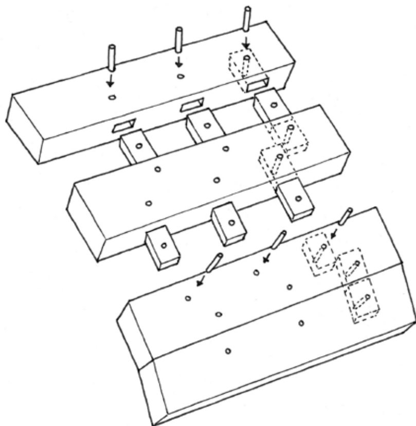
Figure 4.3 Pegged mortise and tenon joints, based on the Uluburun shipwreck, 1300 BCE
